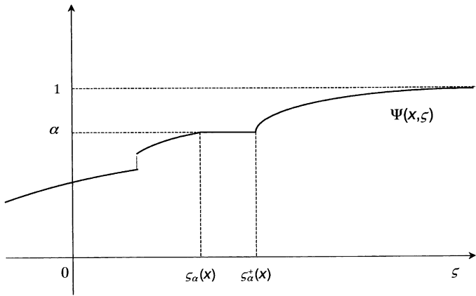
Fig. 2. Equation \Psi(x, \zeta) = \alpha has many solutions in \zeta .
