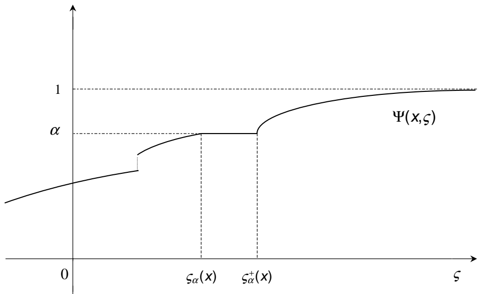
Figure 2: Equation \Psi(x, \zeta) = \alpha has many solutions in \zeta .
