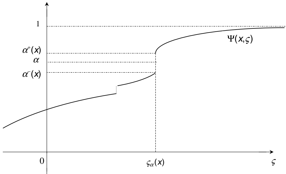
Figure 1: Equation \Psi(x, \zeta) = \alpha has no solution in \zeta .
