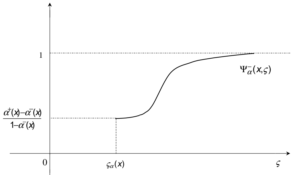
Figure 5: Distribution function \Psi_{\alpha}^{-}(x, \zeta) is obtained by rescaling the function \Psi(x, \zeta) in the interval [\alpha^{-}(x), 1] .
