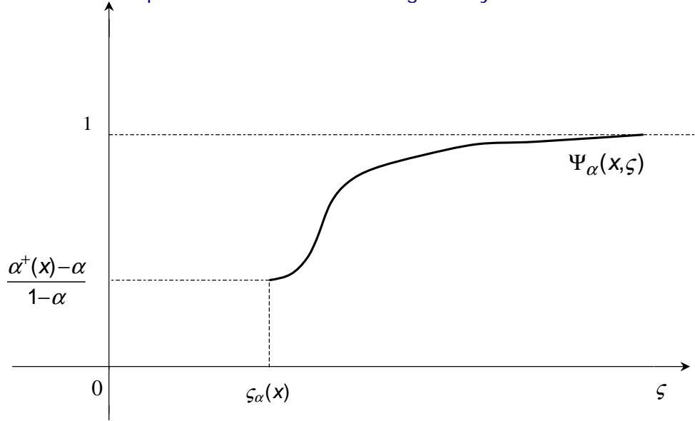
Figure 3: Distribution function \Psi_\alpha(x, \zeta) is obtained by rescaling the function \Psi(x, \zeta) in the interval [\alpha, 1] .
