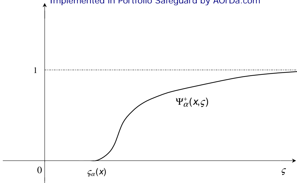
Figure 4: Distribution function \Psi_{\alpha}^{+}(x, \zeta) is obtained by rescaling the function \Psi(x, \zeta) in the interval [\alpha^{+}(x), 1] .
